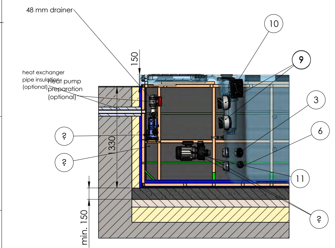
SECTION L-L
